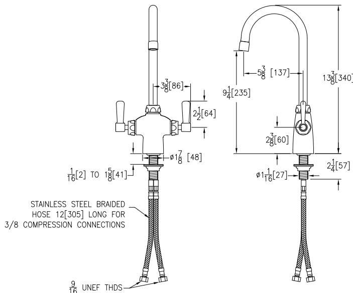
Rough-in/Overview dimensions
