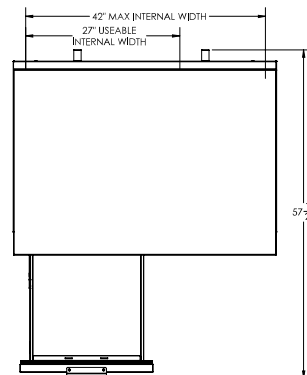
PLAN VIEW
