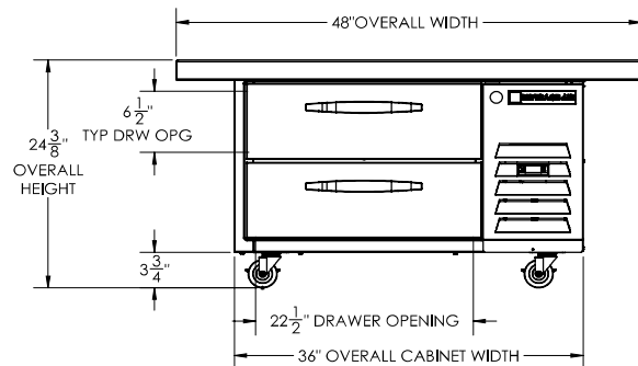
ELEVATION VIEW
