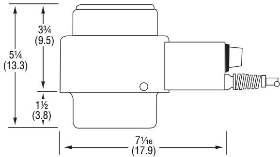
Fully Extended
