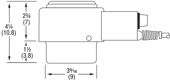
Fully Compressed
