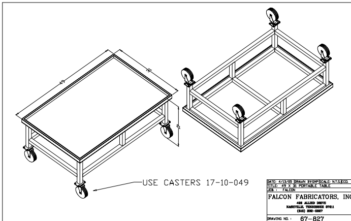
Stand on Casters - 49 x 31 x 21
