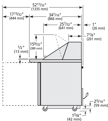
RIGHT VIEW
