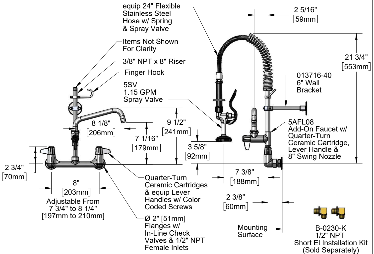
5SP-08 8" Swing Nozzle w/ Laminar Flow Device
