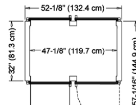
Elevation - R/AHT232NPUT
