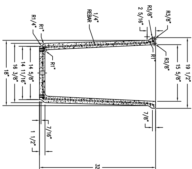
6 SECTION VIEW OF TF1810 WASTE CONTAINER Scale: 1/8" = 1"
