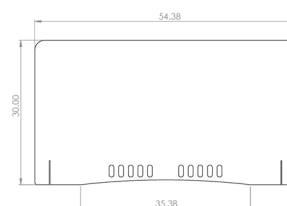
B DOUBLE ACTION STATION SHIELD #CWACT2SHIELD
