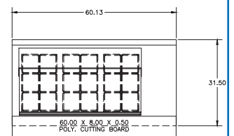
STD4460NP-18M Pan Cutout Configuration
