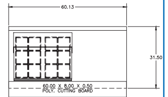
STD4460NP-12M Pan Cutout Configuration
