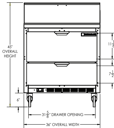
ELEVATION VIEW
