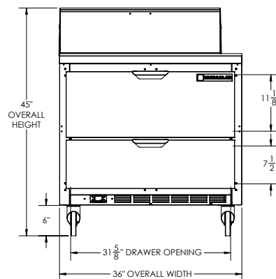
ELEVATION VIEW
