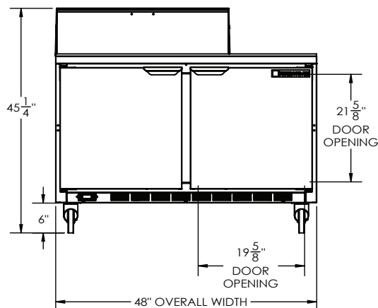
ELEVATION VIEW
