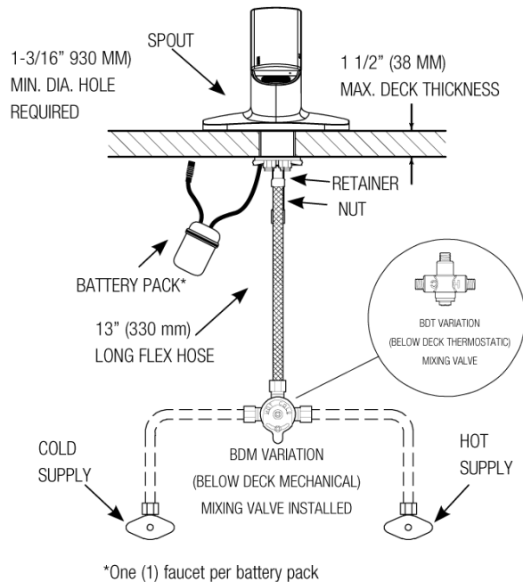
EFX-650.X0X.0000. Faucet with hot and cold water supply
