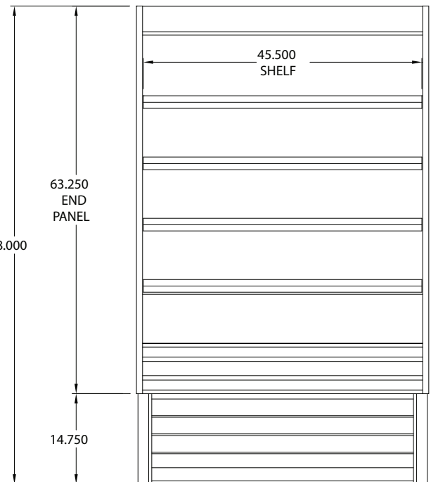
4' FRONT VIEW
