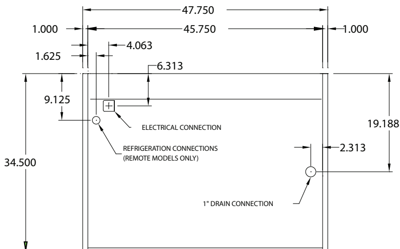
4' FLOOR PLAN VIEW
