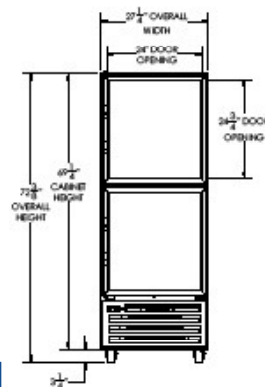
ELEVATION VIEW
