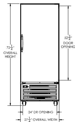
ELEVATION VIEW
