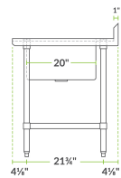
SIDE
