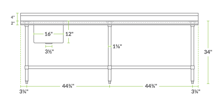
FRONT
