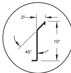
Splash Detail
