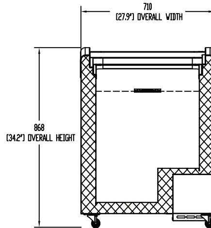
ELEVATION VIEW
