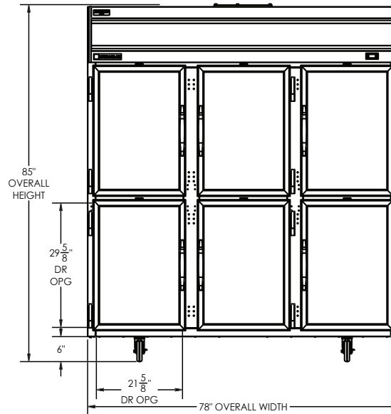
ELEVATION VIEW
