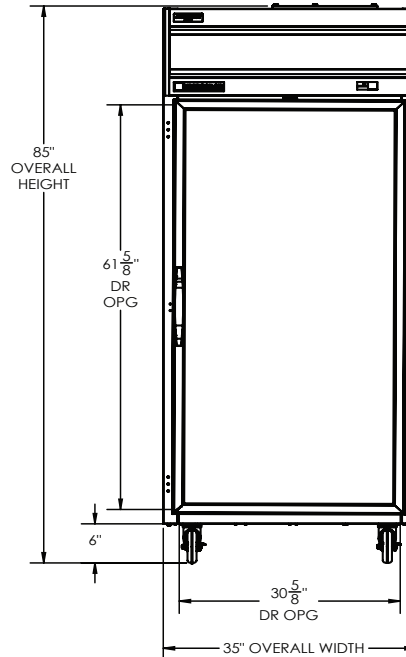
ELEVATION VIEW
