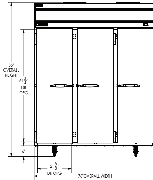
ELEVATION VIEW
