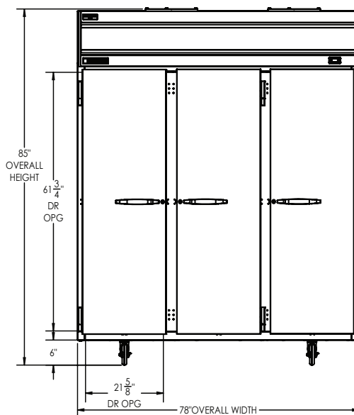
ELEVATION VIEW
