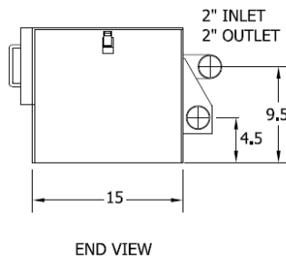
Typical GGXM-15B installation
