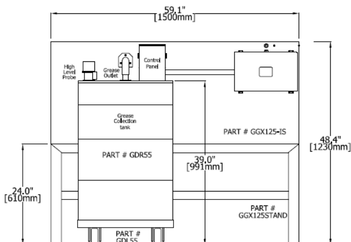
FRONT ELEVATION
