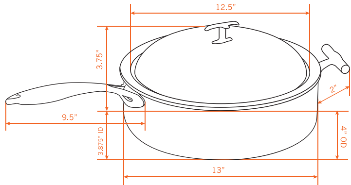
DIMENSIONS FOR 5914, 5914H
