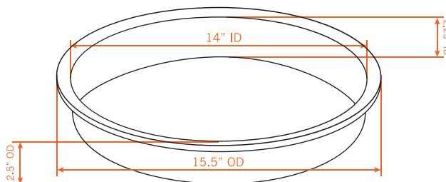
DIMENSIONS FOR 6 QT. FOOD PAN
