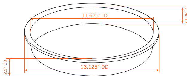
DIMENSIONS FOR 4 QT. FOOD PAN
