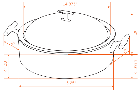
DIMENSIONS FOR 5906, 5906H
