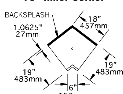
model #WBIC75-19
