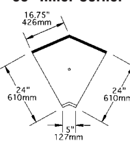
model #WBIC60-24
