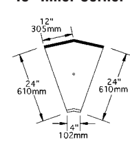
model #WBIC45-24
