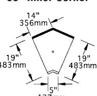
model #WBIC60-19
