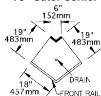
model #WBOC75-19
