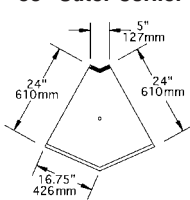
model #WBOC60-24
