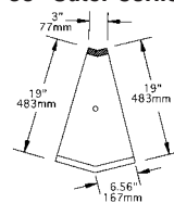
model #WBOC30-19
