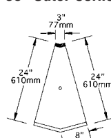
model #WBOC30-24
