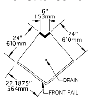
model #WBOC75-24
