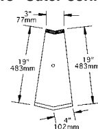
model #WBOC15-19
