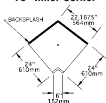
model #WBIC75-24
