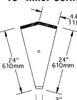
model #WBIC15-24
