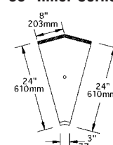
model #WBIC30-24
