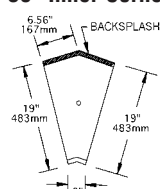
model #WBIC30-19
