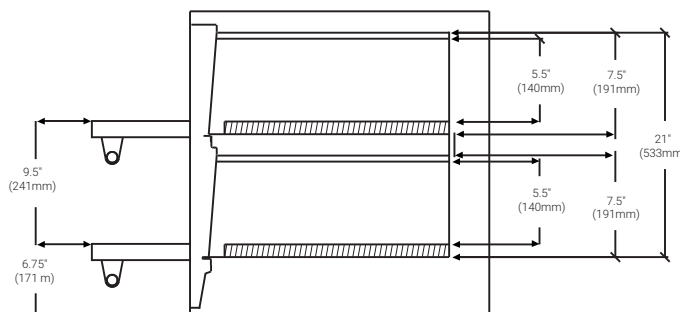
SIDE VIEW / SECTION
