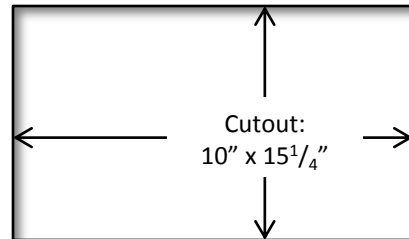
Model #: E1-BS-6OE-W Cutout (Not to scale)
