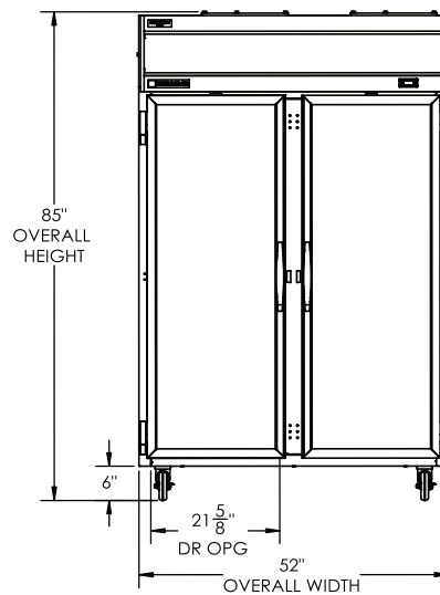
ELEVATION VIEW
