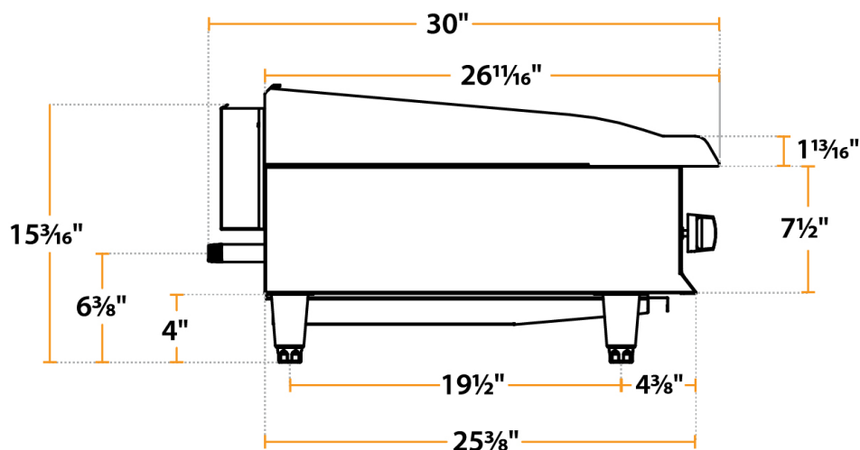
SIDE
