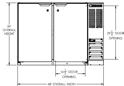
ELEVATION VIEW
