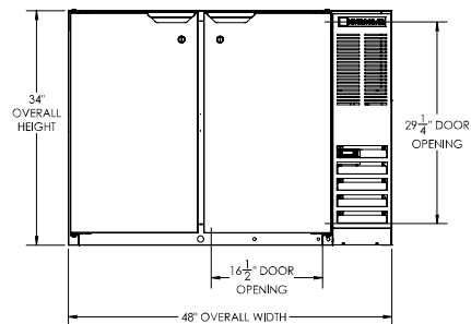
ELEVATION VIEW
