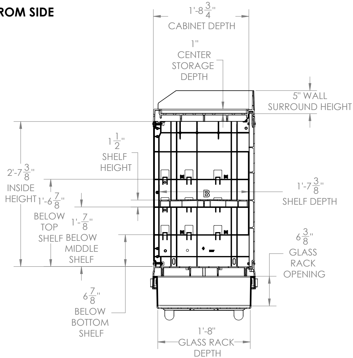
SECTION C-C
