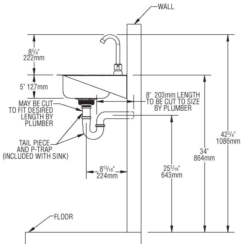
SIDE VIEW
