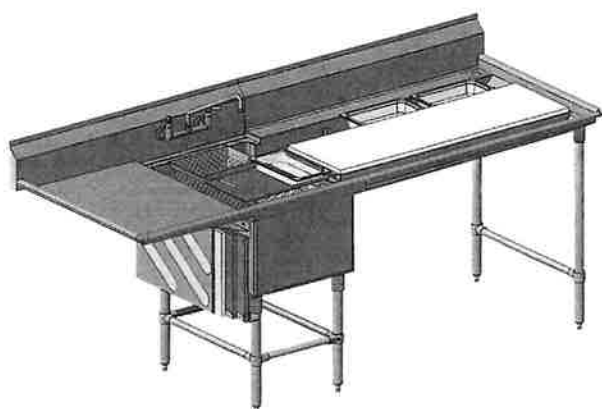
"R" model with trough and prep area at right end (with optional faucet shown)
