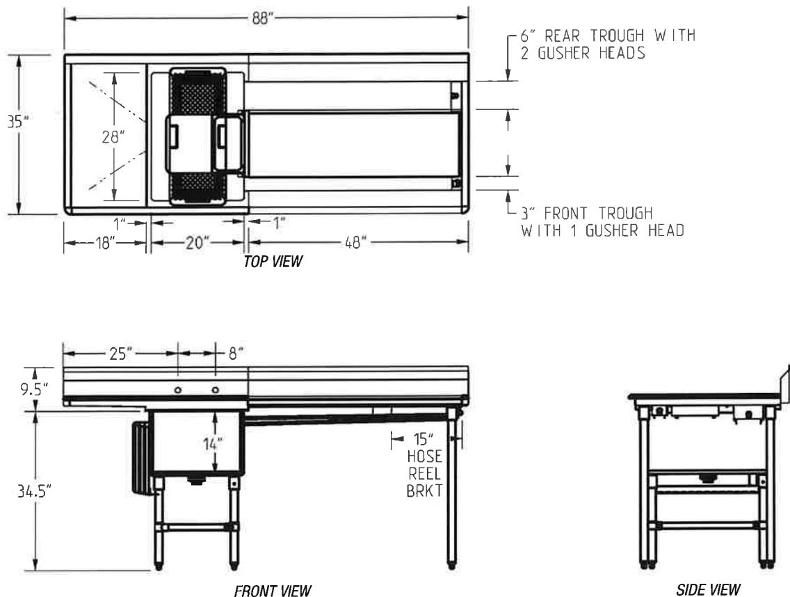
(model #FNP2820-1-18L-48TR shown)
