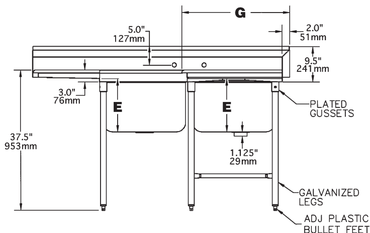
SIDE VIEW
