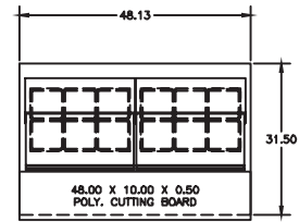
D4448NP-12 Pan Cutout Configuration
