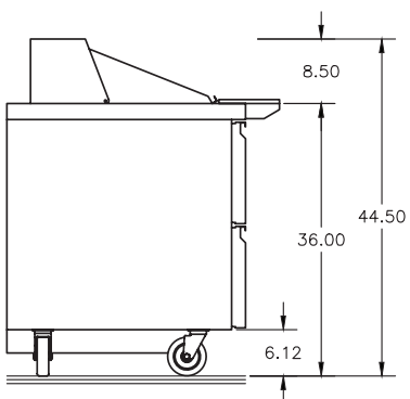
D4432NP-12M Left Side View
