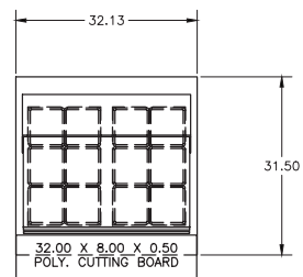
D4432NP-12M Pan Cutout Configuration
