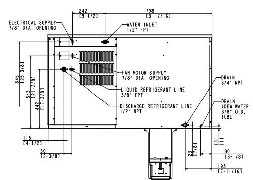
REMOTE AIR-COOLED
