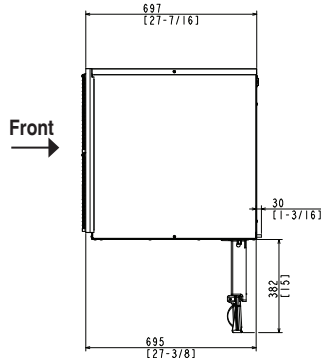
AIR-COOLED
