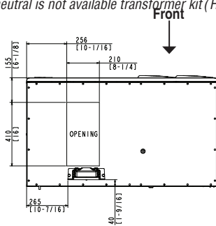
AIR-COOLED
