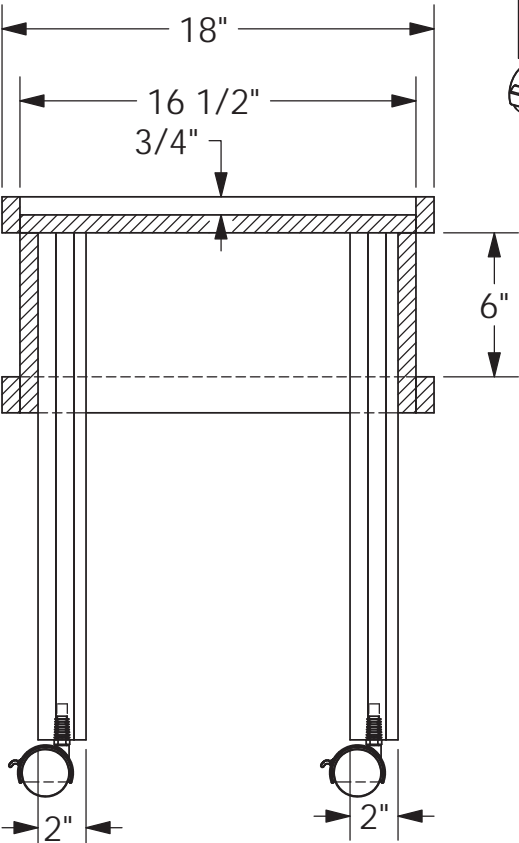
SECTION B-B
