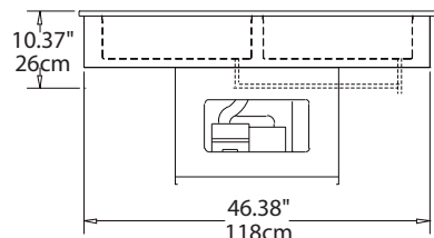
Elevation View 8148-EFNP
