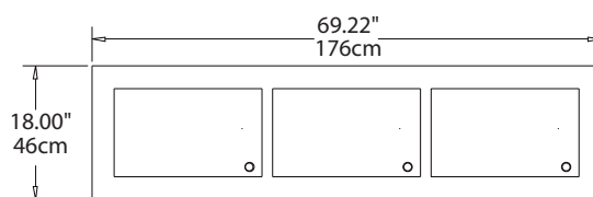
Plan View 8169-EFNP
