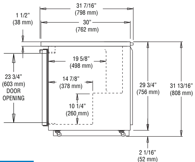
SIDE VIEW
