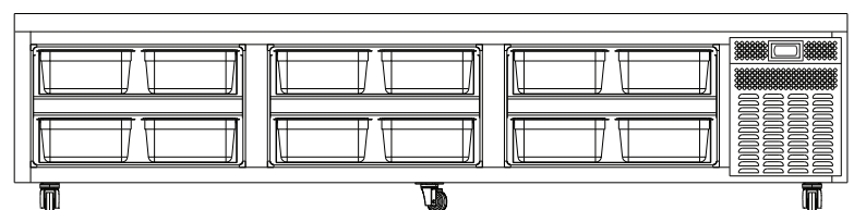
DRAWER PAN CONFIGURATION
