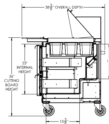
ELEVATION VIEW
