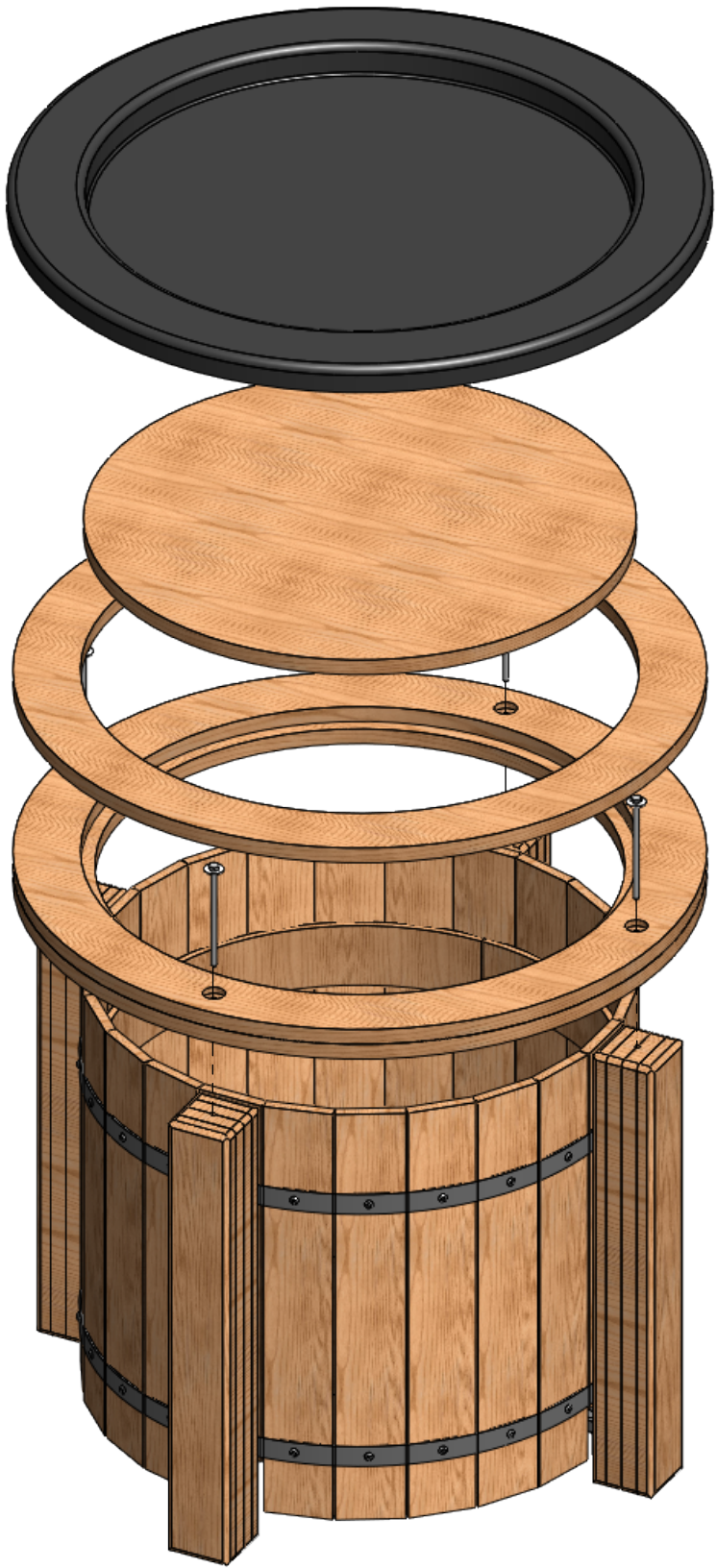
EXPLODED VIEW
