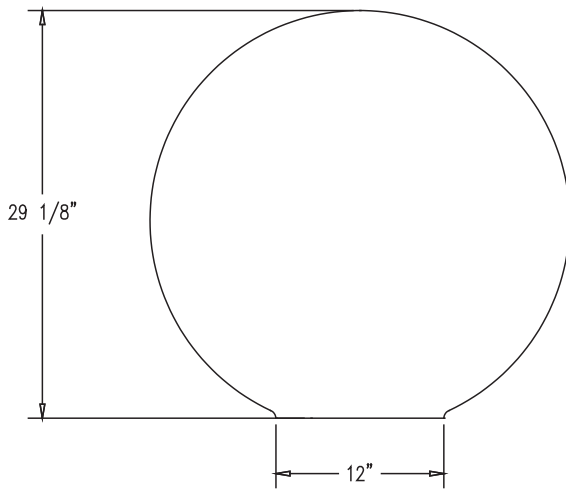
ELEVATION VIEW
