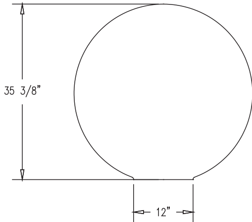
ELEVATION VIEW
